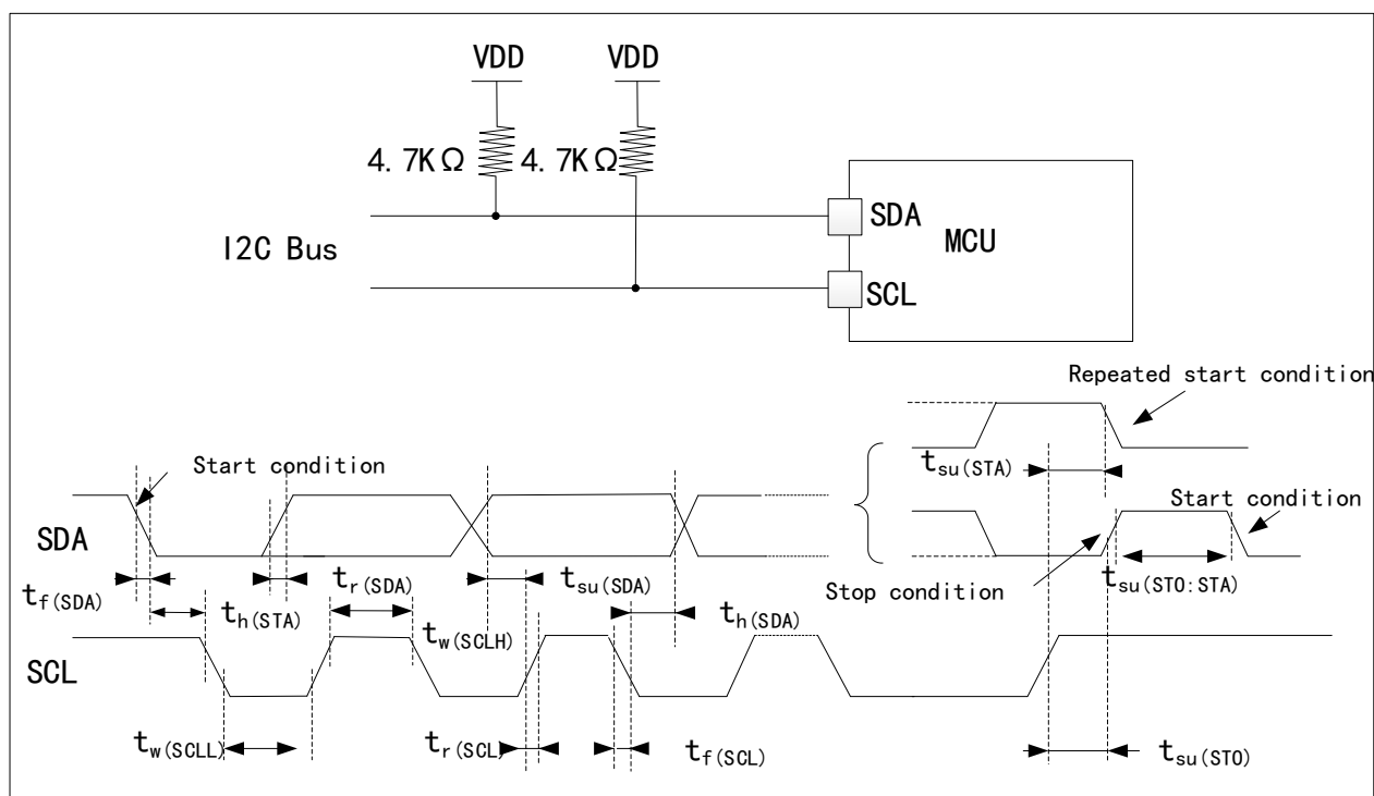
Figure 14 Bus AC Waveform and Measurement Circuit
